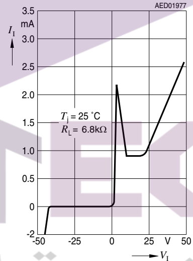
Input Current I_1 versus Input Voltage V_1
